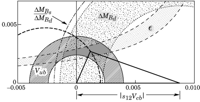
FIG. 3. The unitarity triangle for V_{ud}V_{ub}^* + V_{cd}V_{cb}^* + V_{td}V_{tb}^* = 0 is displayed along with the experimental constraints on V_{ud}V_{ub}^* , which is the upper vertex in the triangle. The constraints following from |V_{ub}| , B-mixing and \epsilon extractions from experimental data are shown in the lightly shaded regions. The experimentally allowed region is indicated by the darkly shaded overlap. The model predicts that V_{ud}V_{ub}^* will lie on the dashed circle; cf. Eq. (21). The particular point on this circle used to draw the triangle shown is obtained from the numbers given in Sec. VI; cf. Eq. (62).
